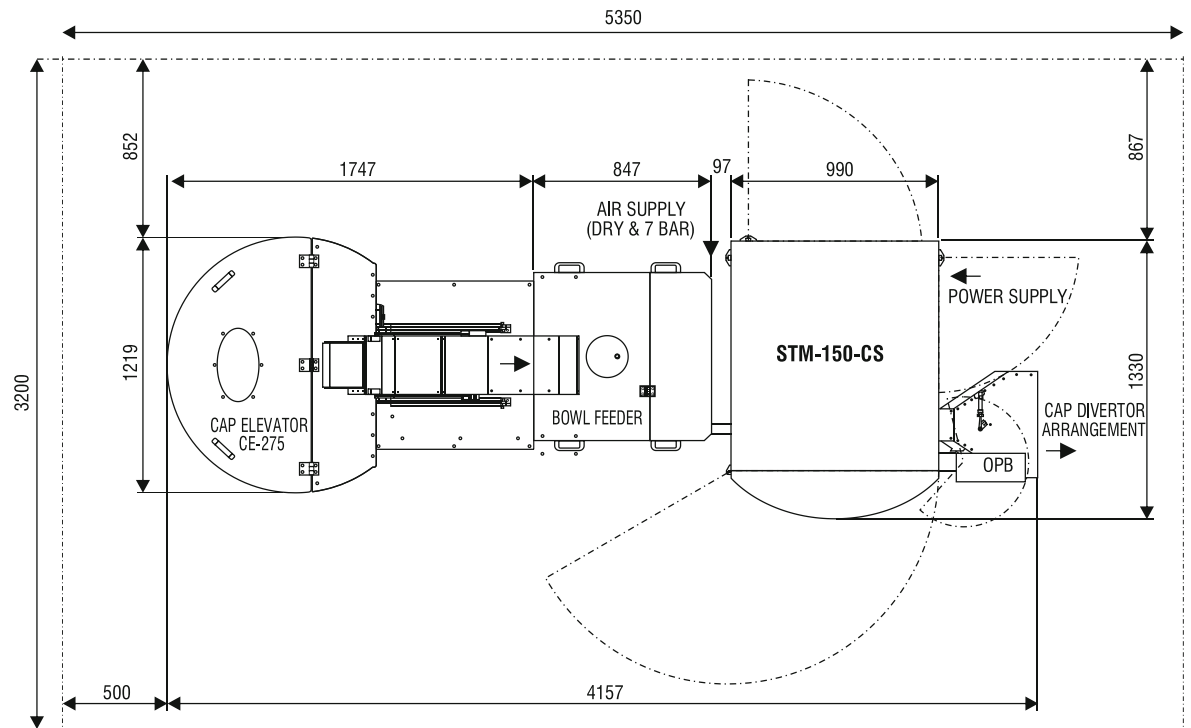
Customize (Decoration) Hot foil stamping on shampoo and conditioner bottle caps
